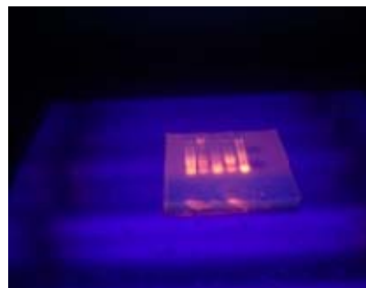
UV Transilluminator
